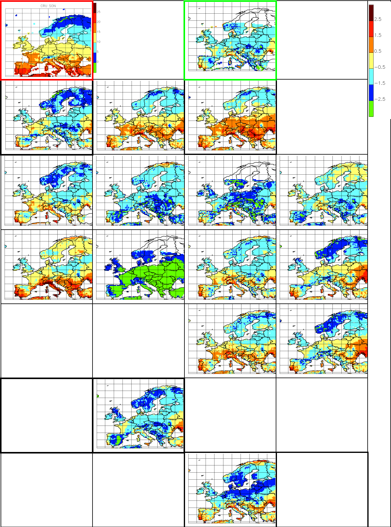
Max Temperature Bias [°C] SON
