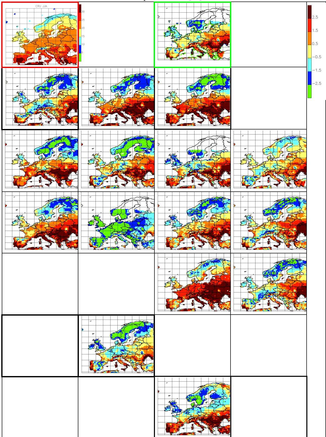
Max Temperature Bias [°C] JJA
