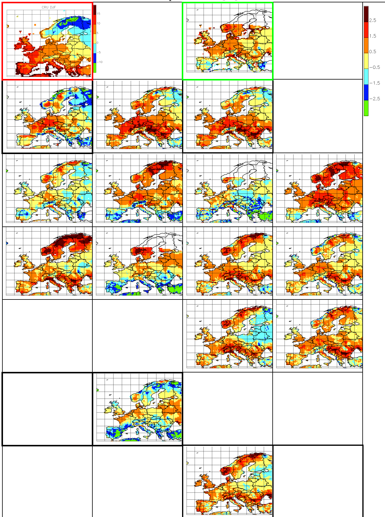
Max Temperature Bias [°C] DJF
