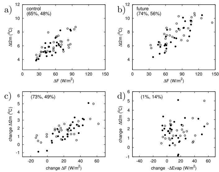
Figure 9. Scatter plot of \Delta t_{2m} against \Delta F = \Delta SW_{net} - \Delta Evap + \Delta LW_{down} for the (a) control integration, and the (b) future integration. Change in temperature variability ( \Delta t_{2m} - Control) against (c) change in \Delta F and (d) change in \Delta Evap . Results are shown for all models and each summer month for SFRA (open circles) and GER (dots). For HadRM3H we set \Delta LW_{down} to the mean of the model ensemble. Between parentheses is the explained variance (%) for (GER,SFRA)
