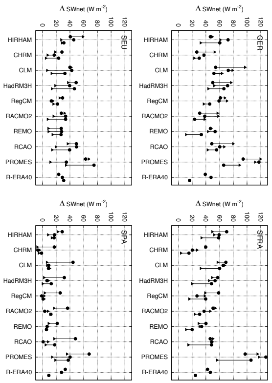
Figure 6. As Fig. 5, but now for \Delta SW_{net} (no observations)
