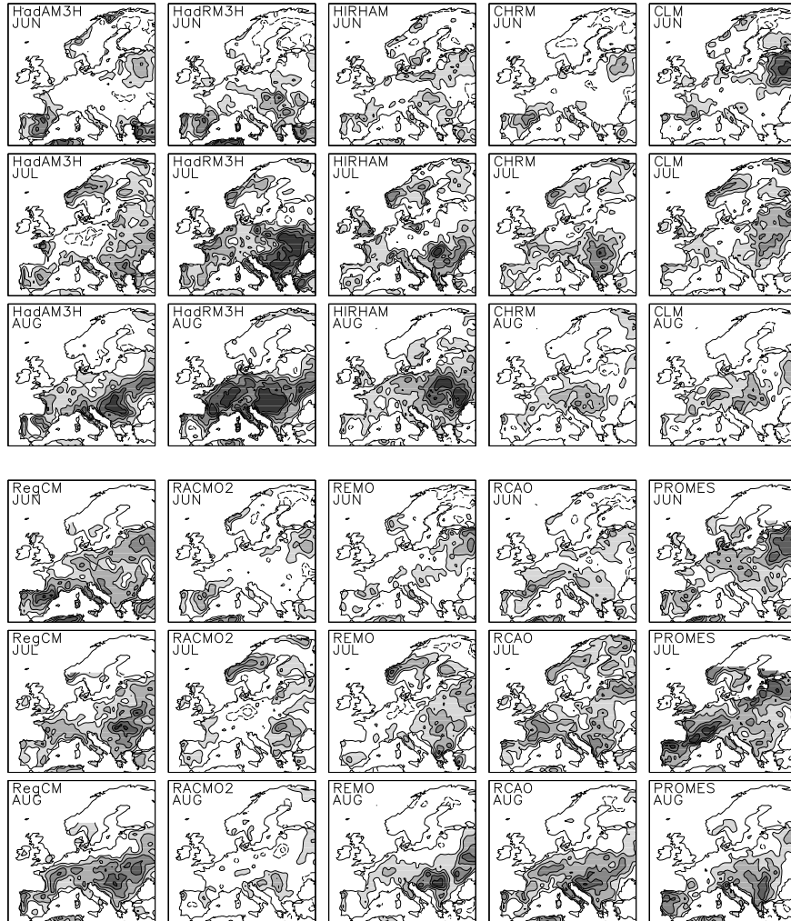
Figure 2. IQR of the monthly mean temperature in HadAM3H and the RCM ensemble. Shown are anomalies to the CRU observations. Shading starts at 0.5 °C with steps of 0.5 °C. Dashed contours denote negative values below -0.5 °C.
