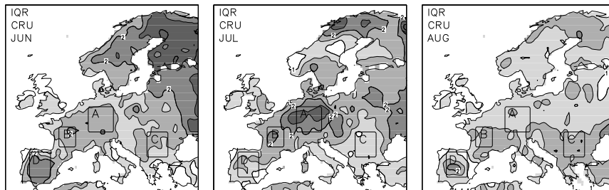
Figure 1. Interquartile range (IQR) of the monthly mean temperature in the CRU observations for June, July, and August. Shading interval 0.5 °C Also shown are four different areas: GER (A), SFRA (B), SEU (C), and SPA (D)
