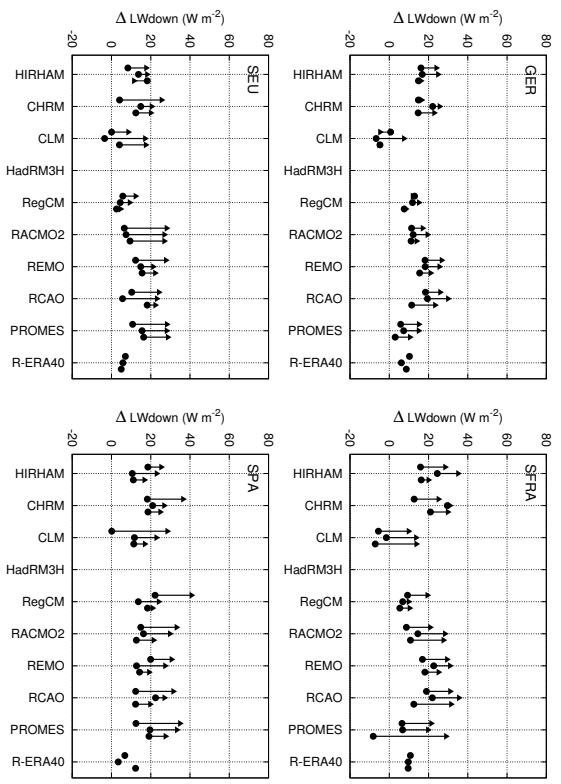
Figure 8. As Fig. 5, but now for \Delta LW_{down} (no observations)
