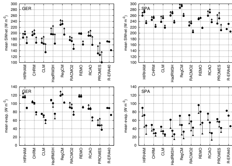
Figure 3. Mean net short-wave radiation and evaporation for GER and SPA. For each RCM results for June, July and August (three consecutive symbols/lines) are shown. Solid dots (triangles) are results for the control (future) integration, with a thick (thin) line denoting increase (decrease) from control to future simulation.
