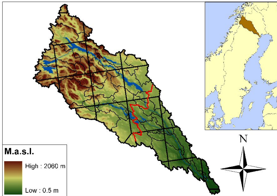
Figure 1. The Lule River Basin including subbasin divisions (thin black lines). The grid delineation is one example of an RCM resolution at about 50 km (RCAO). The red line shows the division into northwest and southeast used for subarea calculation of the delta factors. The background colors indicate elevation.
