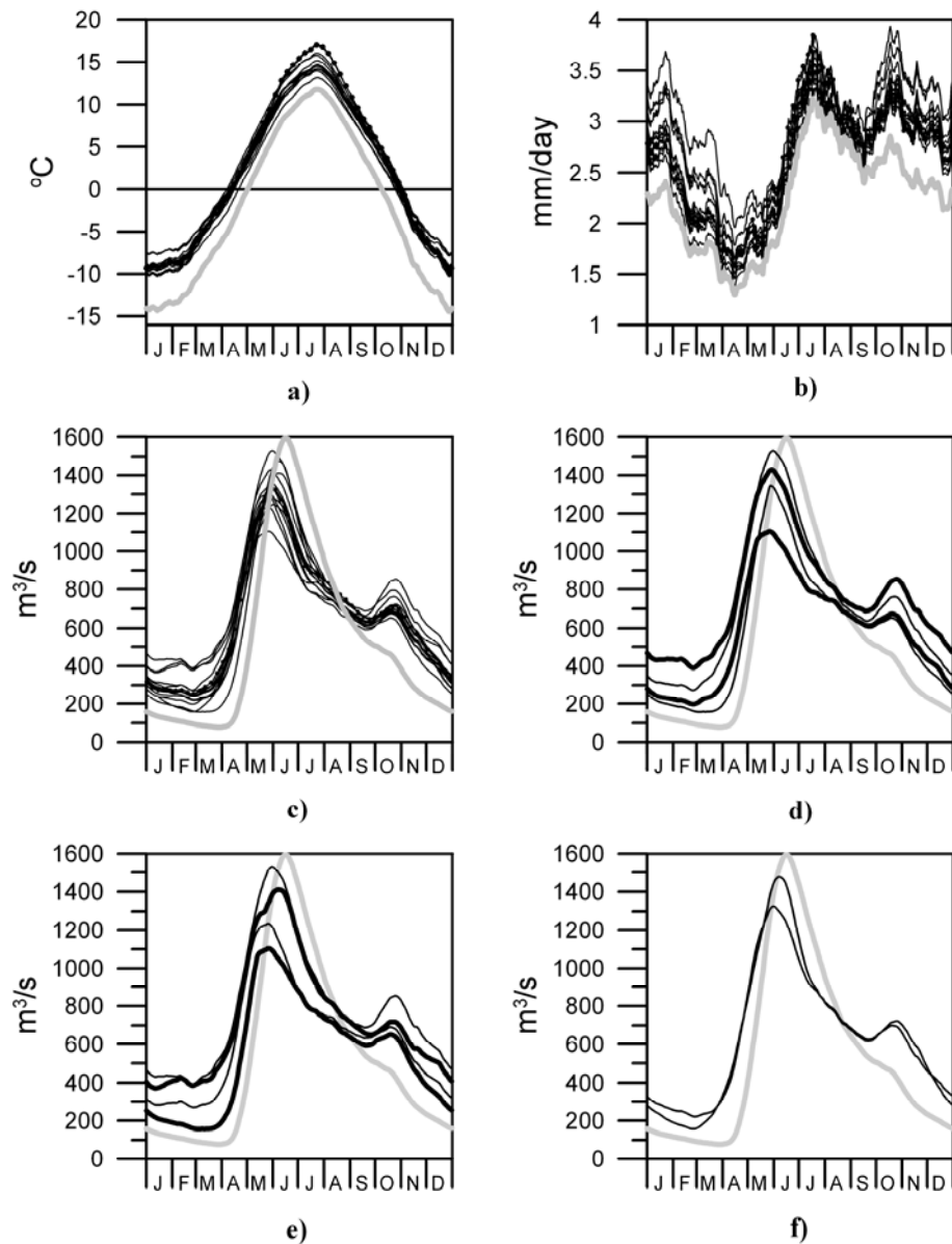
Figure 2. Basinwide a) 2 m temperature, b) precipitation, and c-f) river discharge for HBV hydrological simulations using the delta approach with an ensemble of 15 climate model simulations for the Lule River Basin. Meteorological inputs a) and b) represent future conditions and are observations from 1982-1998 plus climate scenario changes. The grey lines are the actual observations used for the reference simulation; the dotted line in a) shows GCM results from HadAM3H. Mean river discharge for all simulations is shown in c). The remaining plots show the ensemble range for, d) all A2 (thick lines) and all B2 (thin lines) simulations, e) all HadAM3H (thick lines) and all ECHAM4/OPYC3 (thin lines) simulations, and f) the two 25 km simulations.
