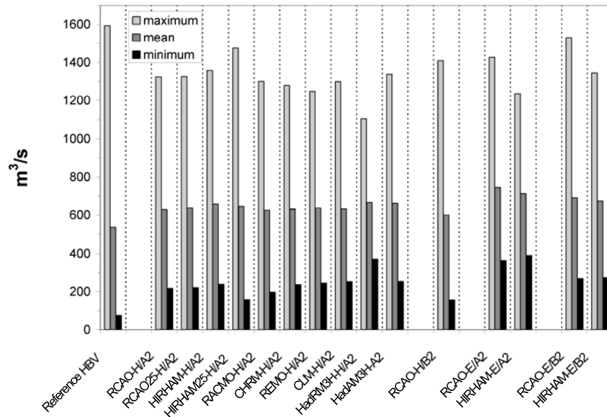
Figure 3. Mean maximum, mean annual and mean minimum river discharge for Lule River from HBV hydrological simulations using the delta approach. The simulations are grouped according to boundary GCM and scenario. For comparison, the HBV reference simulation for 1982-1998 is shown.
