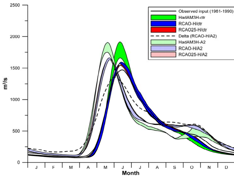
Figure 4. a) Mean river discharge from HBV hydrological simulations using observed input (black solid) and the delta change approach (black dotted) compared with direct use of climate model input from HadAM3H (green solid), RCAO (blue solid) and RCAO25 (red solid). The corresponding scenario simulations are dashed lines. b) Mean river discharge from HBV hydrological simulations using observed input (black solid) and the delta change approach (black dotted) compared with simulations using scaled climate model output. The filled intervals between lines show differences resulting from scaling on annual and monthly basis.
