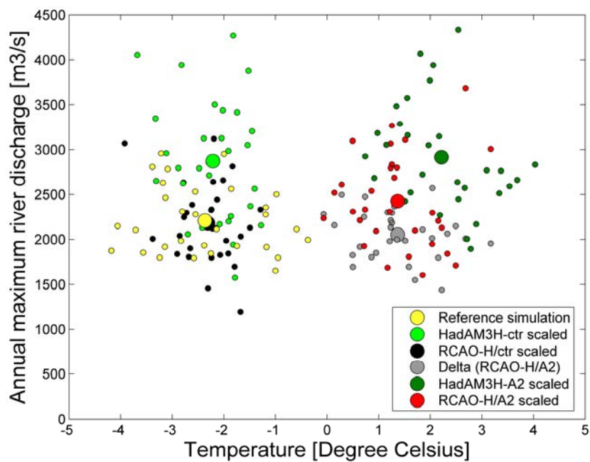
Figure 6. a) Mean annual river discharge and b) maximum annual river discharge plotted against mean annual temperature for the HBV reference simulation (1961-1990), annually scaled RCAO-H/ctr, HadAM3H-ctr, corresponding scaled A2 scenarios, and the corresponding A2 delta scenario. Small dots show individual years and large dots are the respective mean values for all years.
