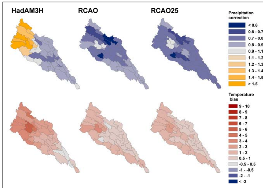
Figure 5. Deviation from observed precipitation (corrected for undercatch) and temperature for HadAM3H, RCAO and RCAO25 in the Lule River Basin.
